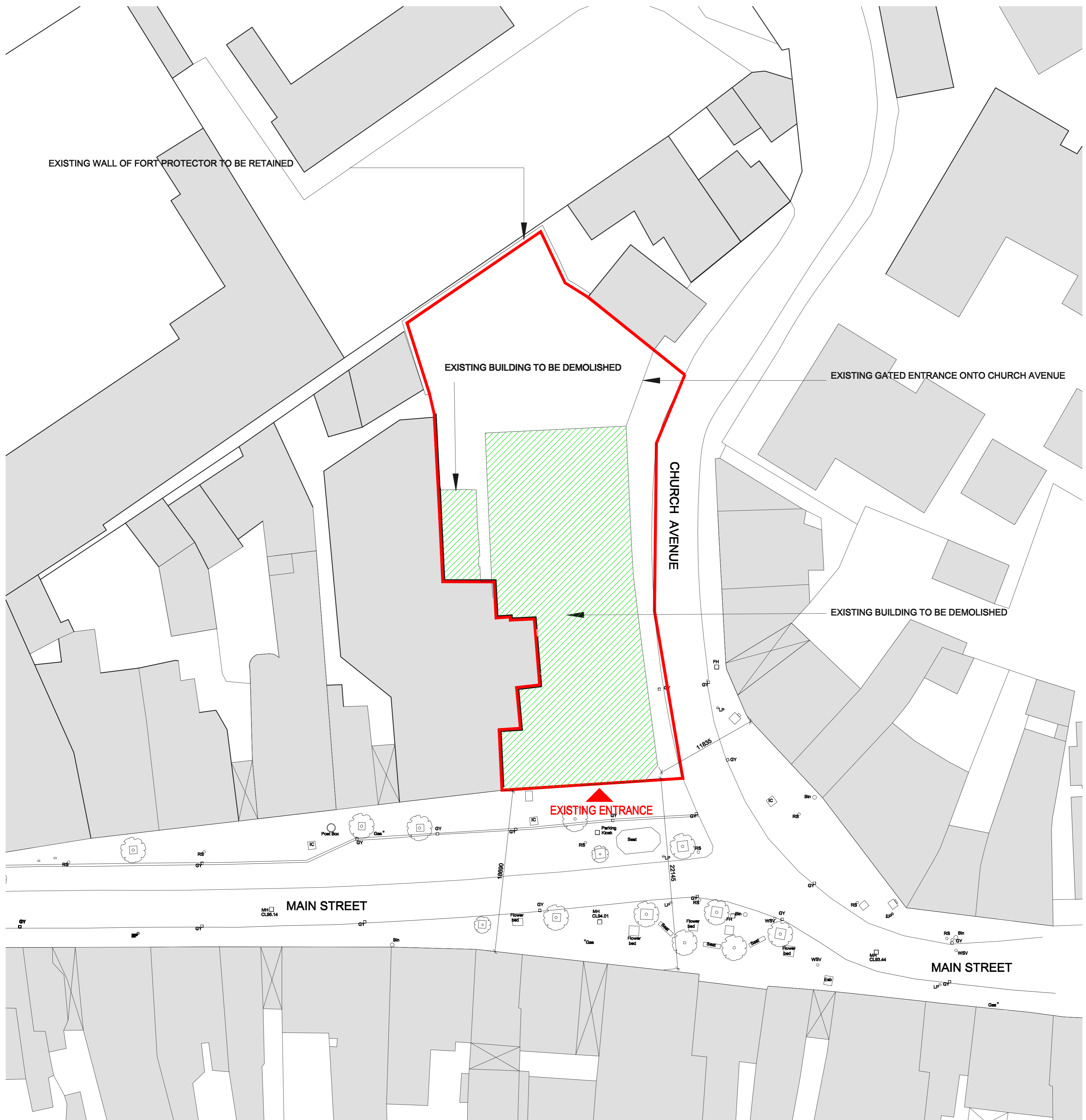
EXISTING SITE PLAN scale 1:250
