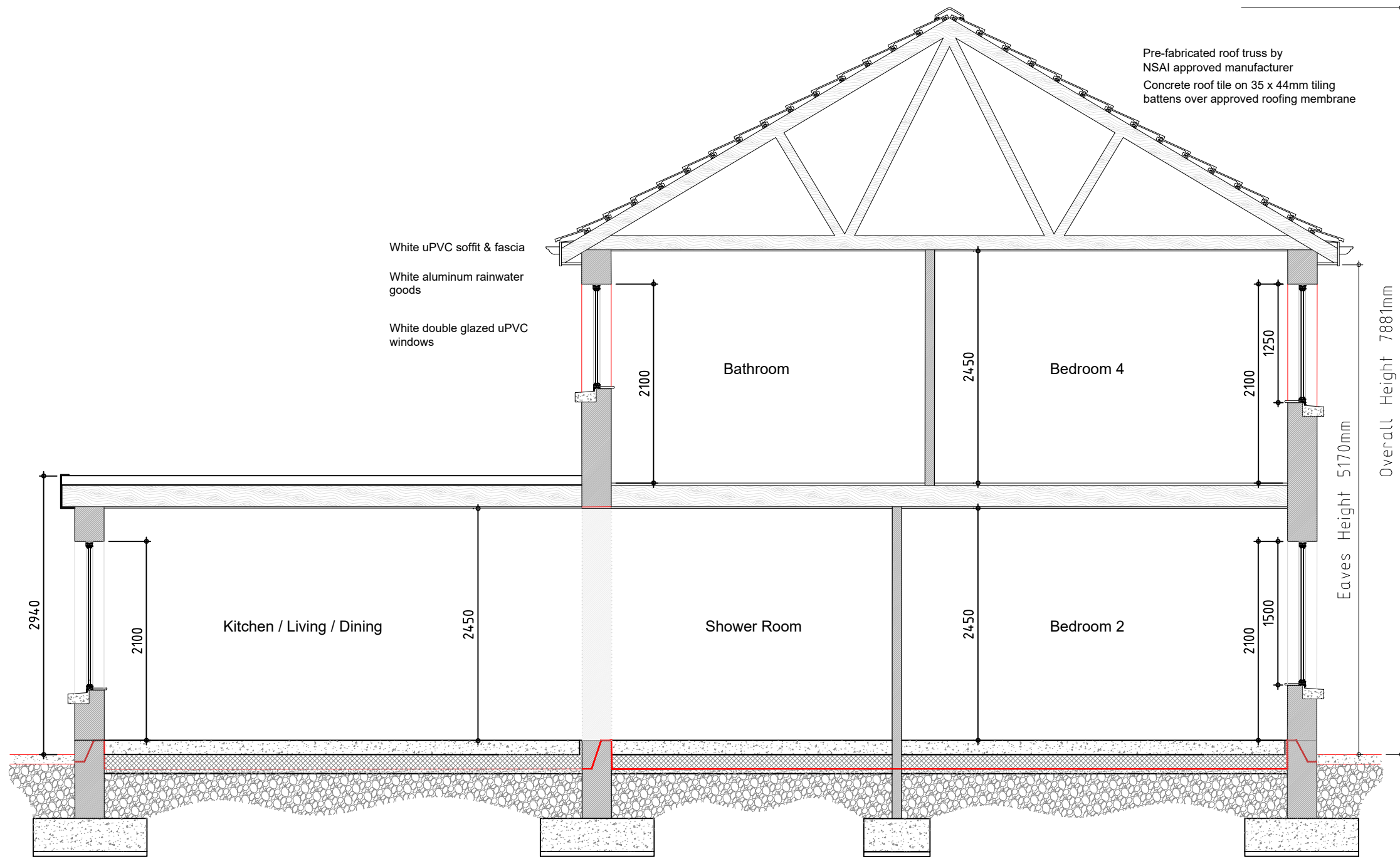
01 Section A - A
