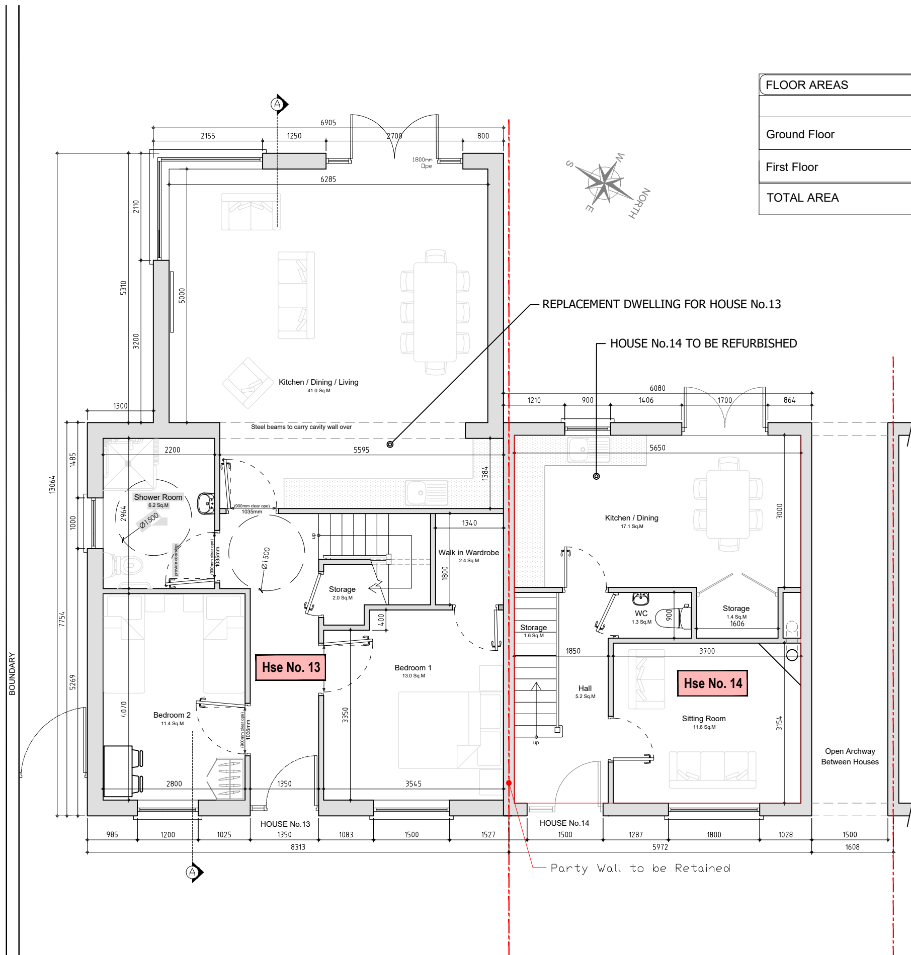
01 Proposed Ground Floor Plan Scale: 1:75
