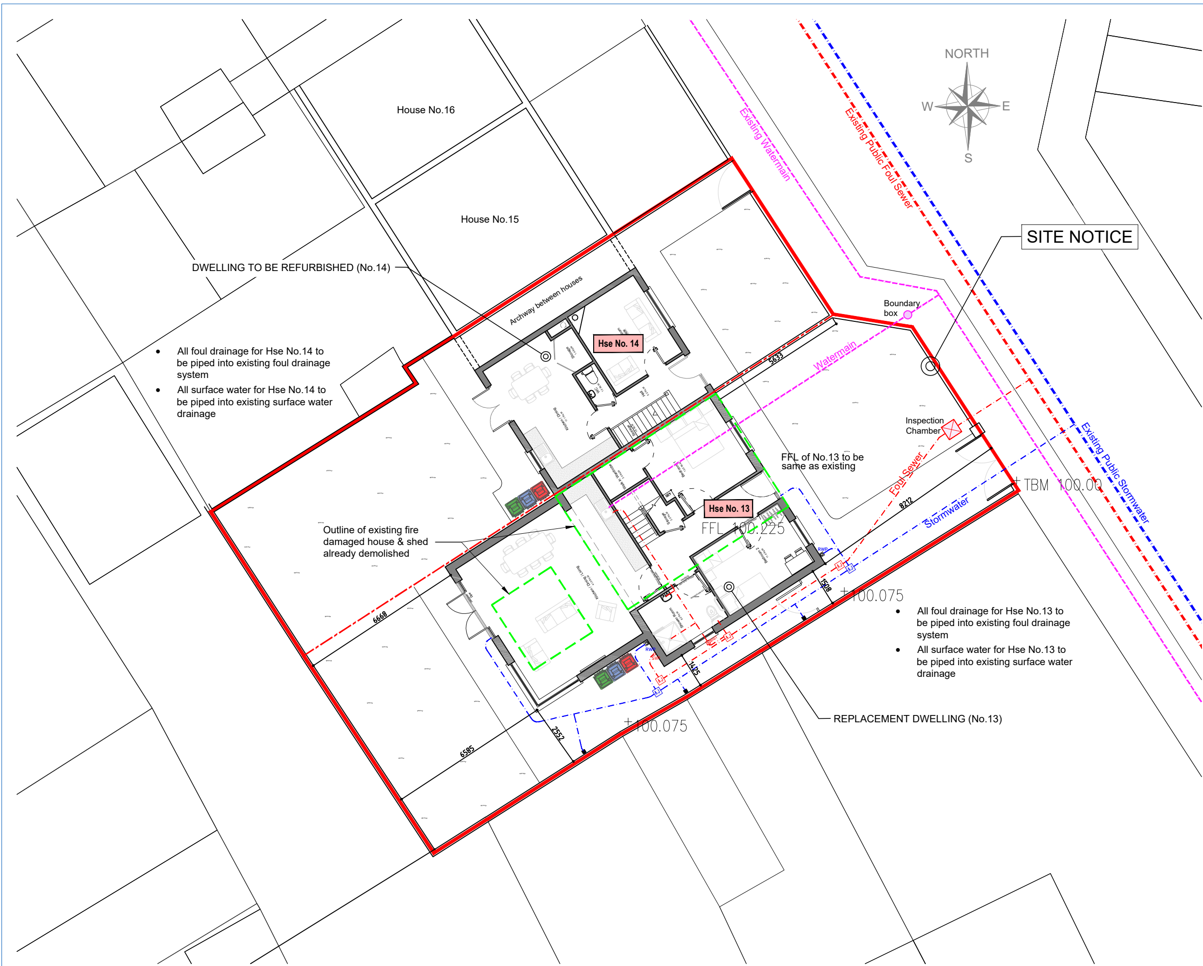
1 Site Layout Plan Scale 1:150
