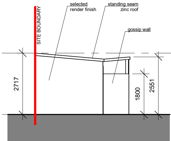
1 Side (East) Elevation 1 : 100
