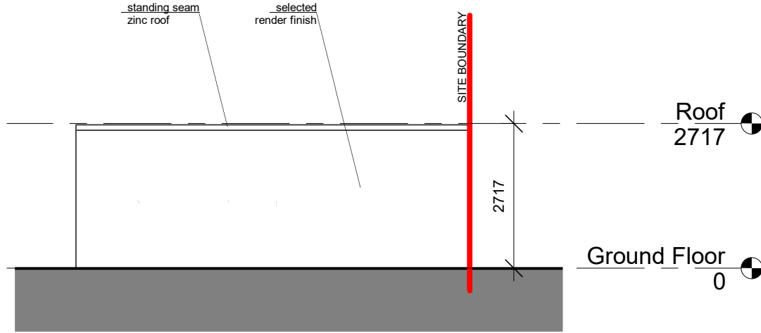
2 Rear (South) Elevation 1 : 100
