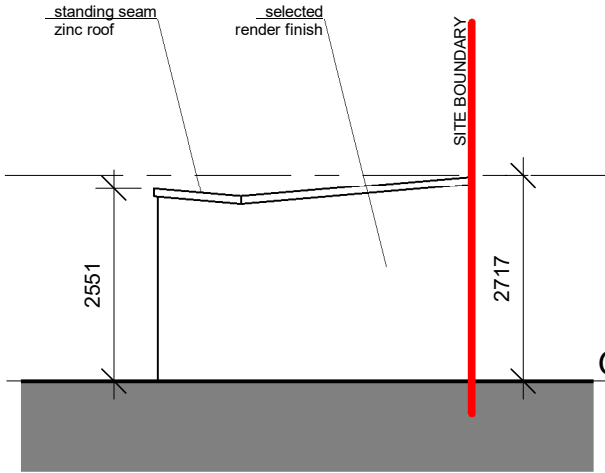
4 Side (West) Elevation 1 : 100
