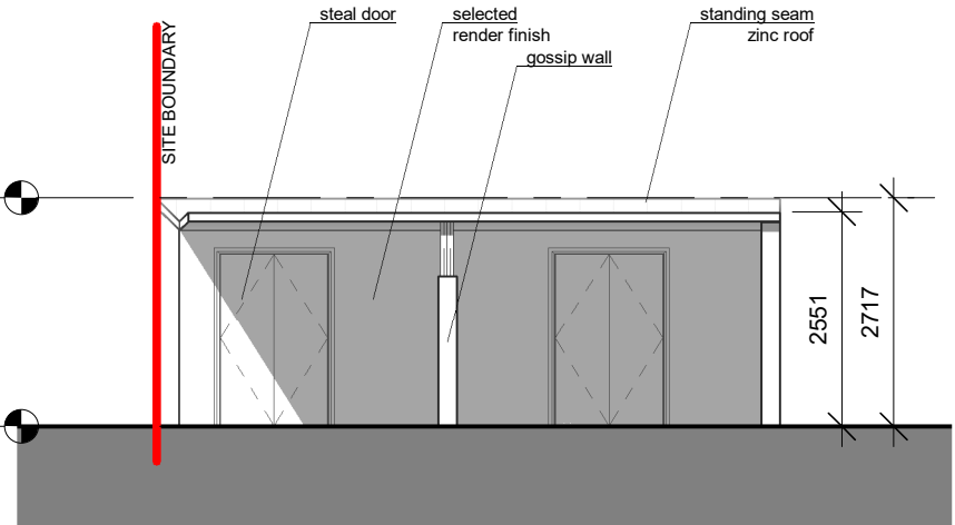
3 Front (North) Elevation 1 : 100
