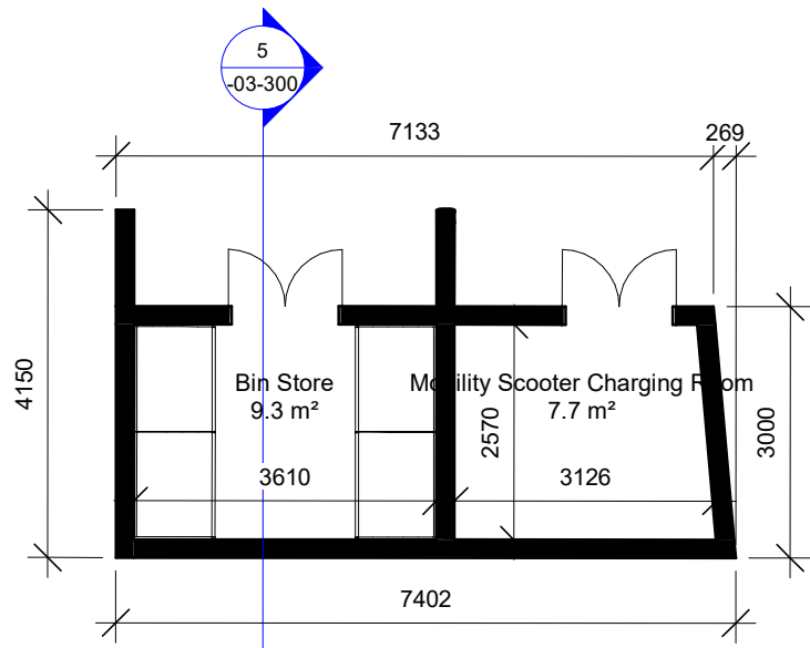
6 Ground Floor 1 : 100
