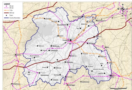
Map 7: Transmission Network in County Laois
